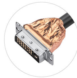
DVI (18+1)P Male 360° Copper Foil Wrap Soldering Shield
