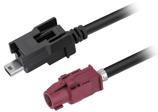
Automotive Cable HSD to USB Mini-B Assembly AWG26, LEONI
