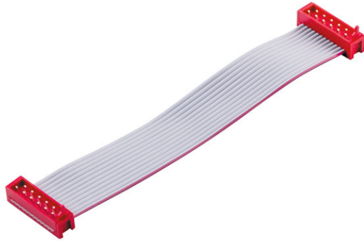
IDC Flat Cable IDC 11P Male to Male AWG28, UL Listed (UL2651)
