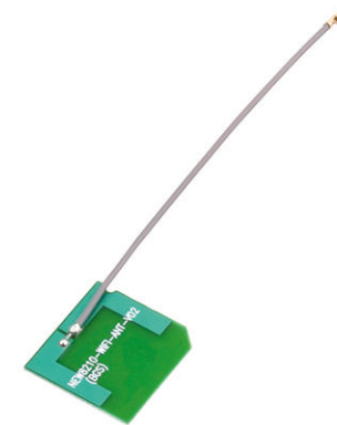
Bluetooth Antenna Long Range WiFi Antenna I-PEX MHF 20278-001R-13 to PCB RF1.13 Cable
